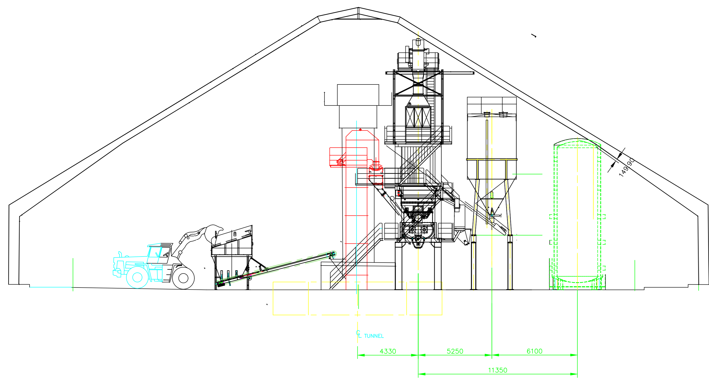
Section On "C" - "C"
